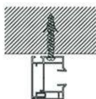
Ceiling installation
